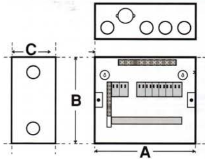
Dimensions (mm)
