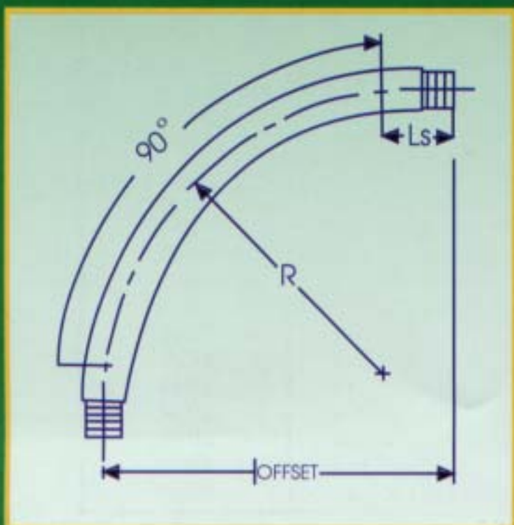
ELBOW
