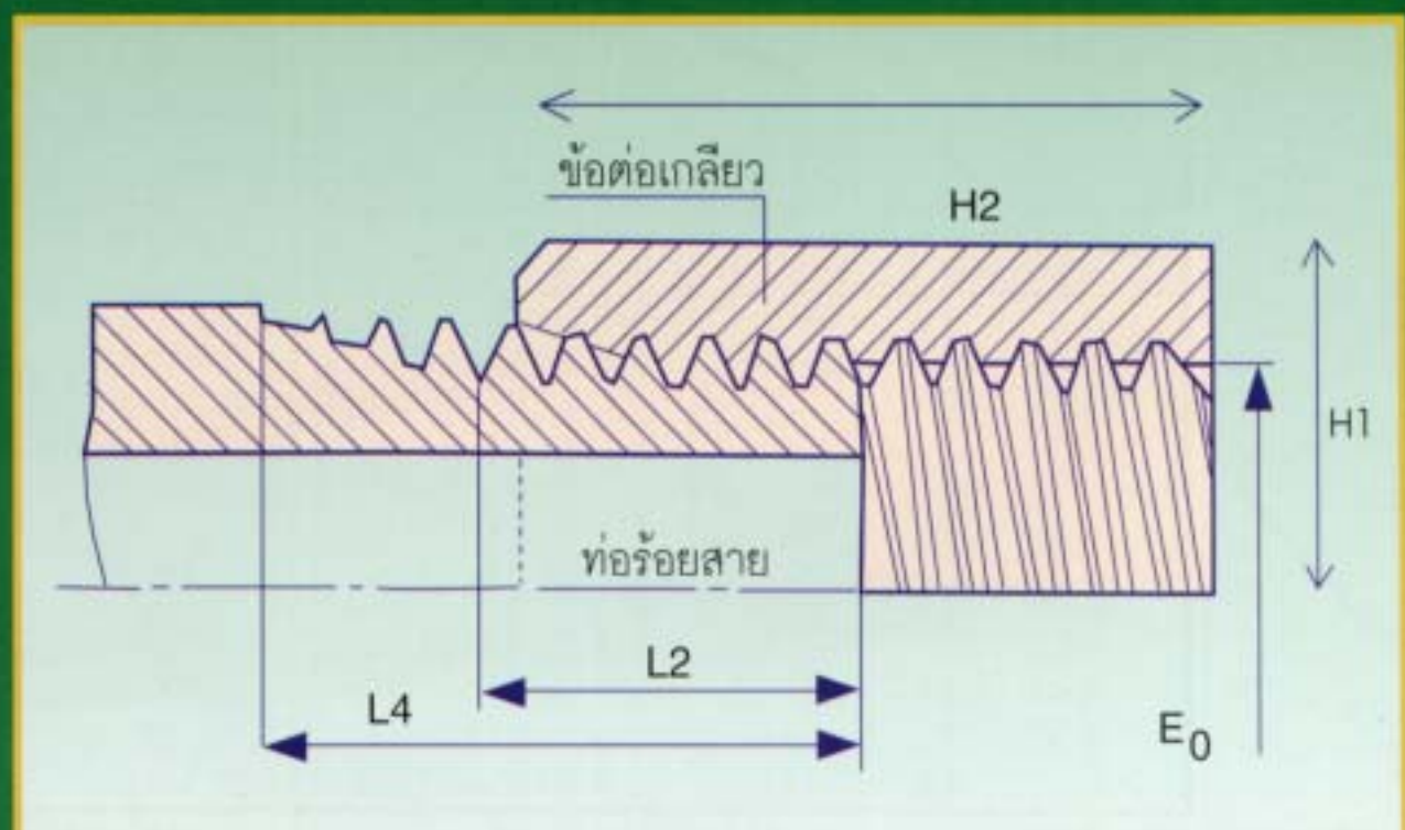
COUPLING
